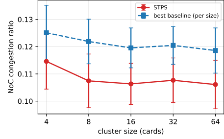
Figure 11: NoC congestion ratio versus cluster size (bursty, task count scaled with cards, 5 seeds, 95 % CI). STPS stays below the per-size best baseline from 4 to 64 cards, holding a stable 8–12 % relative advantage.
